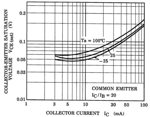
Fig. 10.20 RN1102 V_{CE(sat)} - I_C
