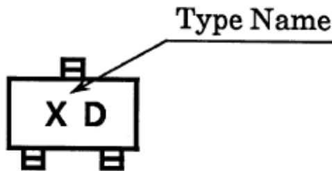
Fig. 9.4 Marking RN1104
