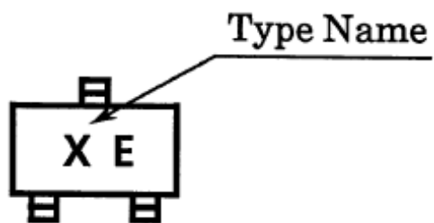
Fig. 9.5 Marking RN1105
