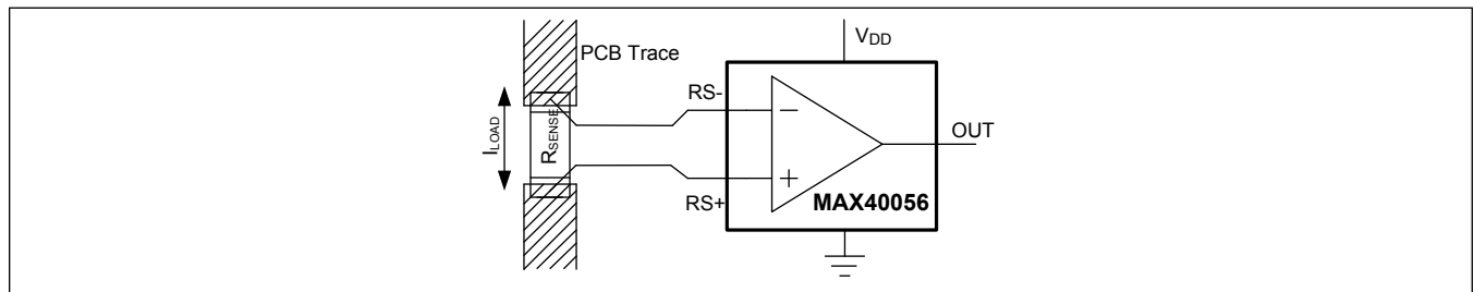
Figure 4. Kelvin Sensing
