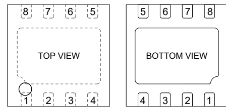
Figure 3-2. Pin Configuration (DFN8L)
