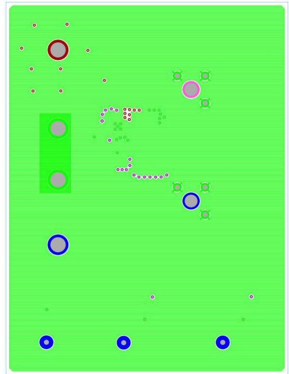
FIGURE 6. LAYER 2 PCB
