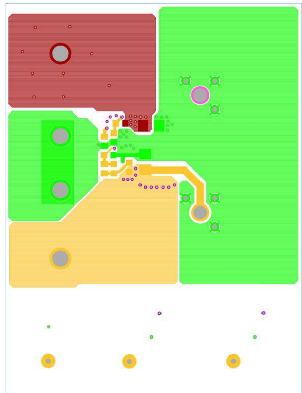
FIGURE 8. LAYER 4 PCB
