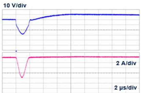
Figure 10. ESD response to ISO 7637-3 pulse 2a: -85 V
