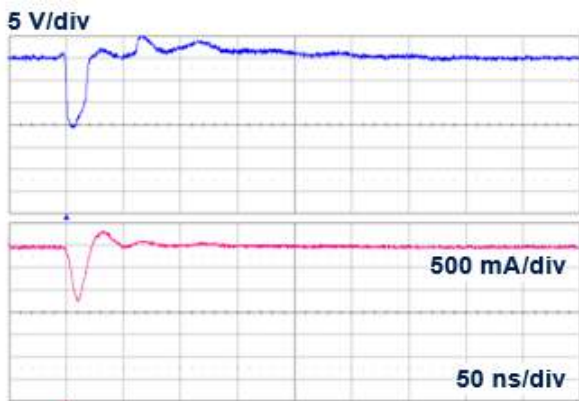
Figure 8. ESD response to ISO 7637-3 pulse 3a: -150 V
