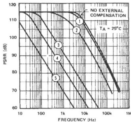
PSRR vs FREQUENCY (OP-06B, OP-06E)
