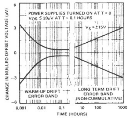
OFFSET VOLTAGE DRIFT WITH TIME
