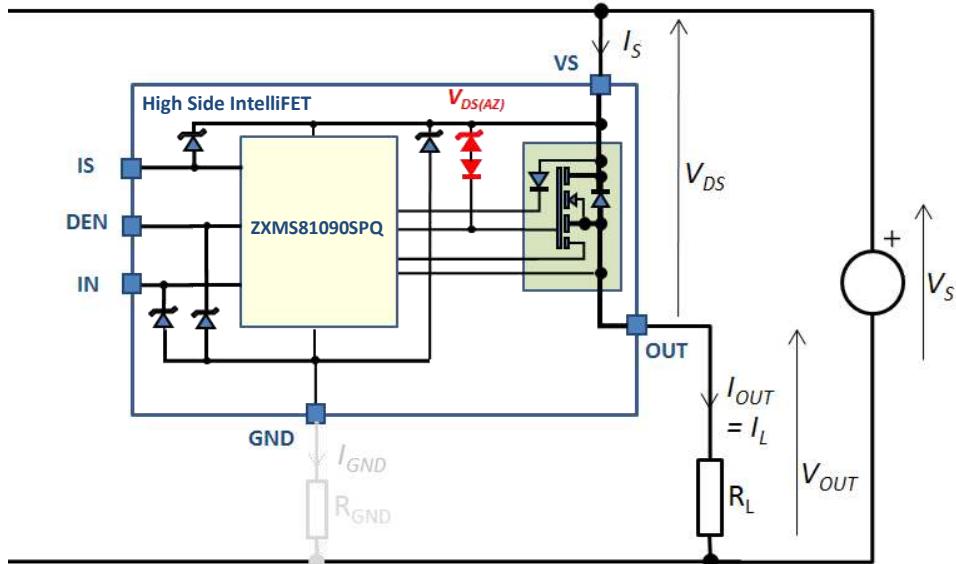
Figure 6. Output Clamp
