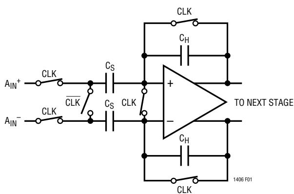
Figure 1. Input Sample-and-Hold Amplifier
