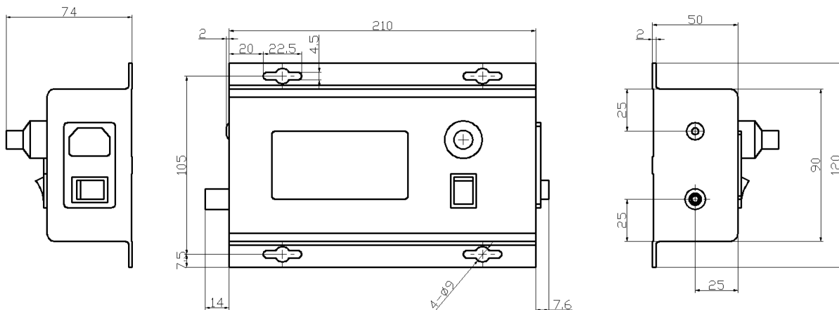
Figure 9. Dimensions for AHVACN5KV5MABT
