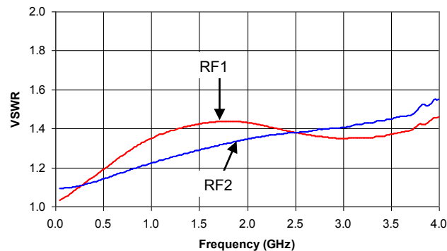
VSWR - 15.5 dB Attenuation vs. Frequency
