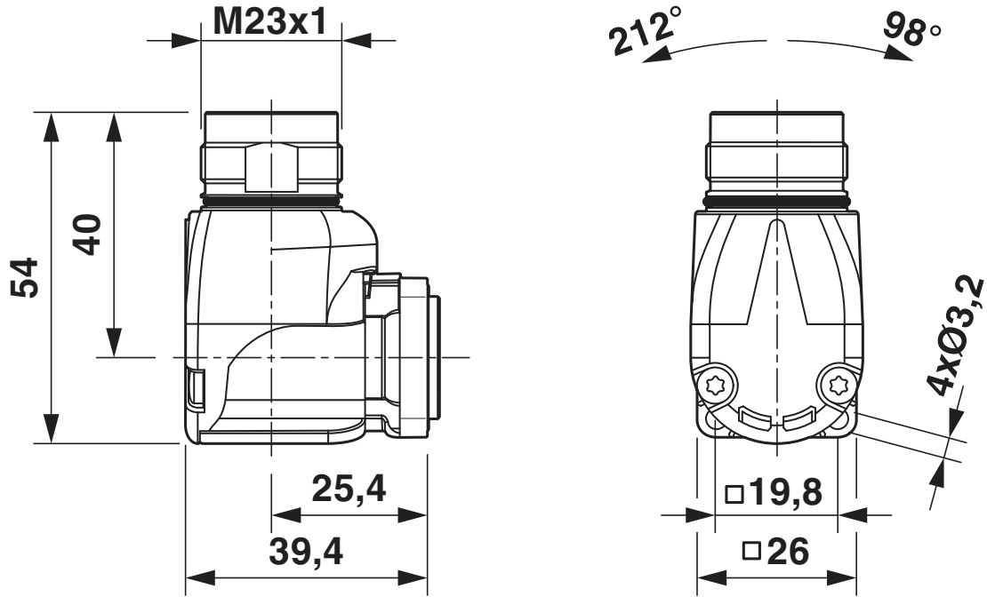
Dimensioned drawing
