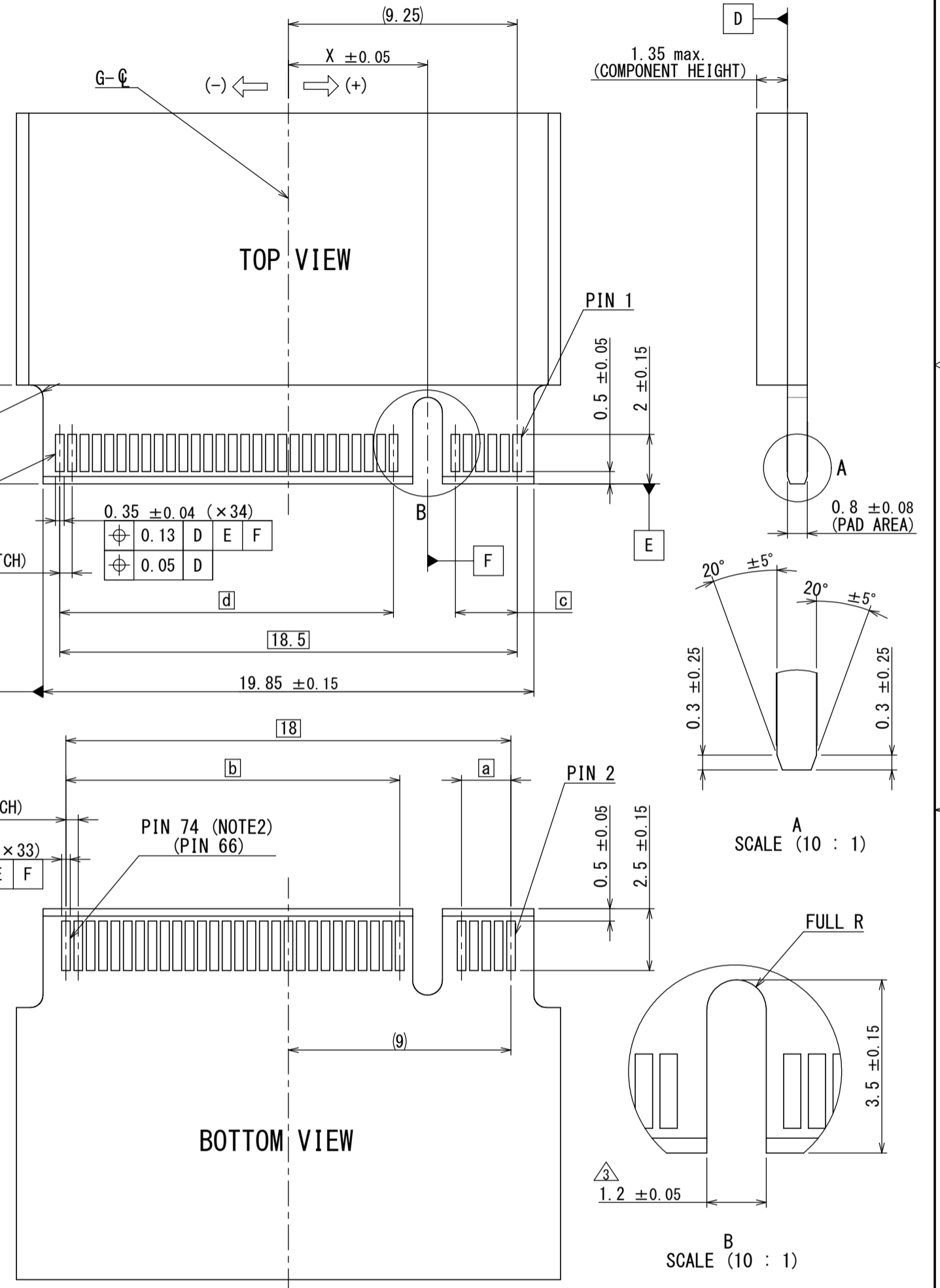
APPLICABLE MODULE DIMENSION (REF.) SCALE (5:1)
