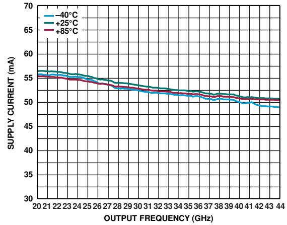
Figure 19. Supply Current ( I_{D02} ) vs. Output Frequency at Various Temperatures, 5 dBm Drive Level
