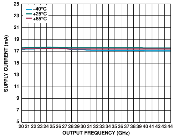
Figure 18. Supply Current ( I_{D01} ) vs. Output Frequency at Various Temperatures, 5 dBm Drive Level
