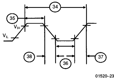
Master Clock Timing
