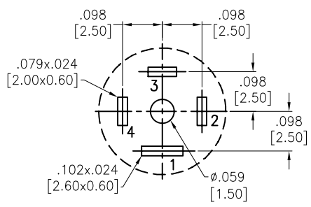
RECOMMENDED PCB LAYOUT (COPPER SIDE VIEW)
