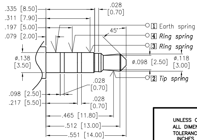
MATE PLUG
