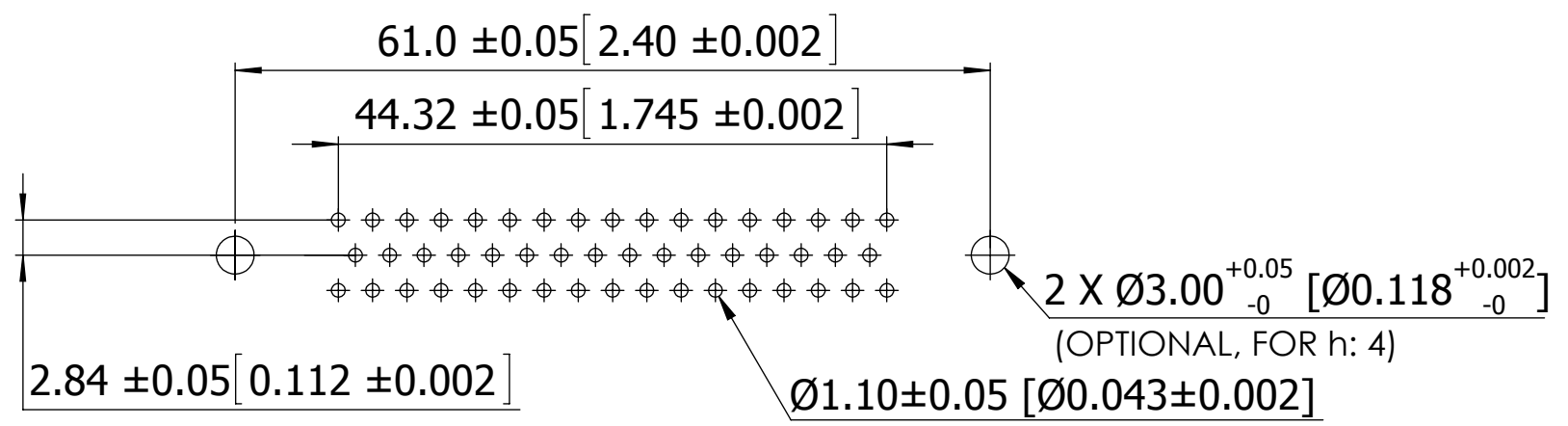
RECOMMENDED PCB LAYOUT 50 POSITIONS ( PN EXAMPLE: SDS155-PRW2-M50-QN00-1 )
