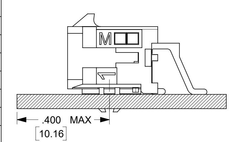
LOCATION DETAIL (SEE NOTE #9)
