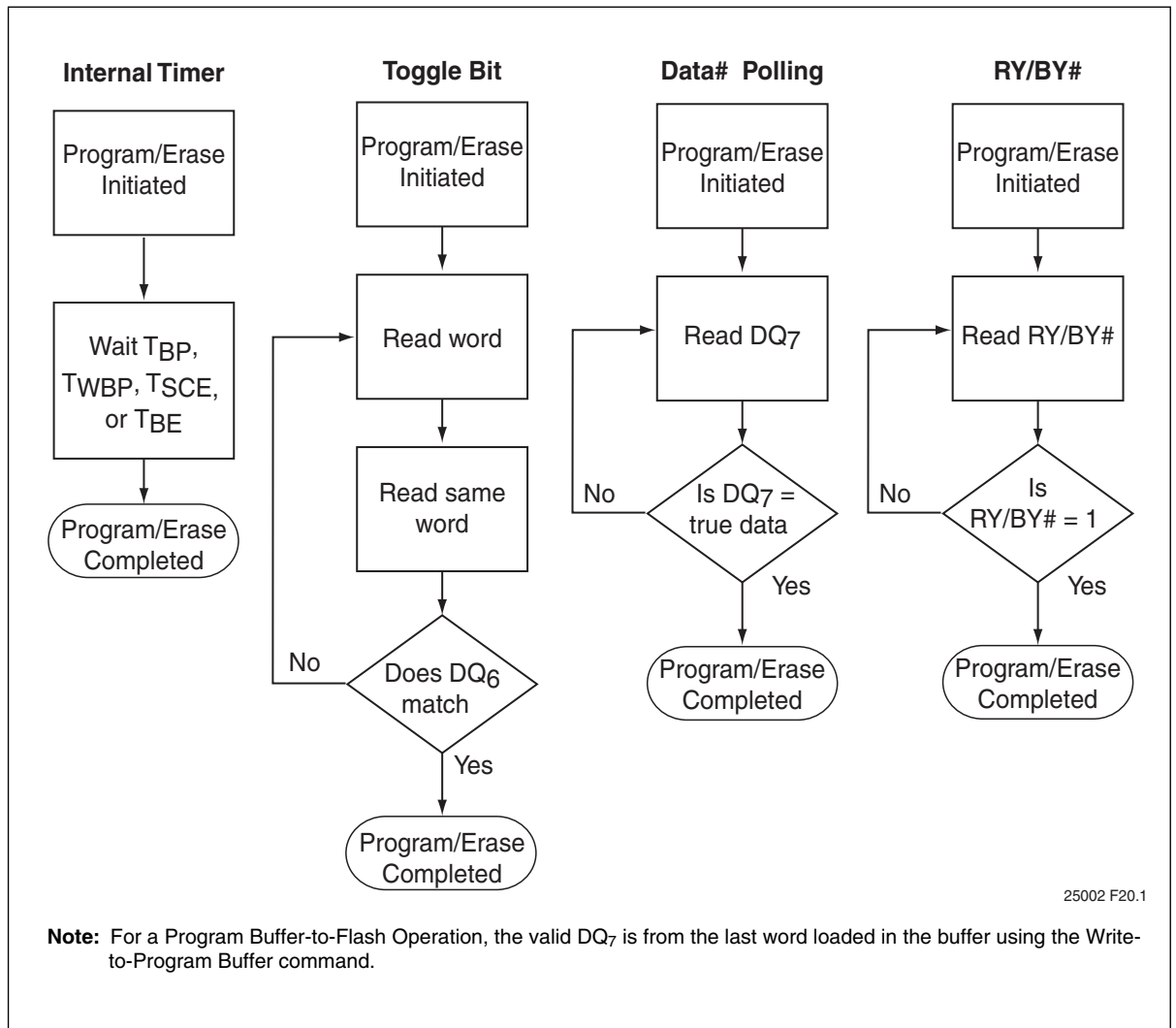
Figure 25: Wait Options
