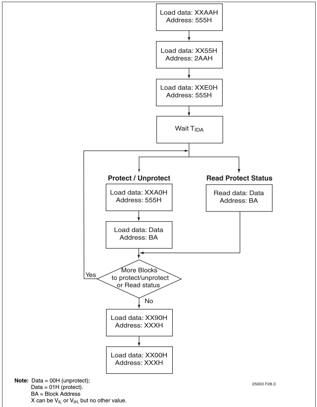
Figure 30: Volatile Block Protection
