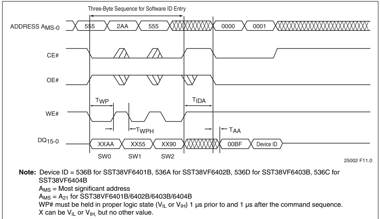
Figure 15: Software ID Entry and Read
