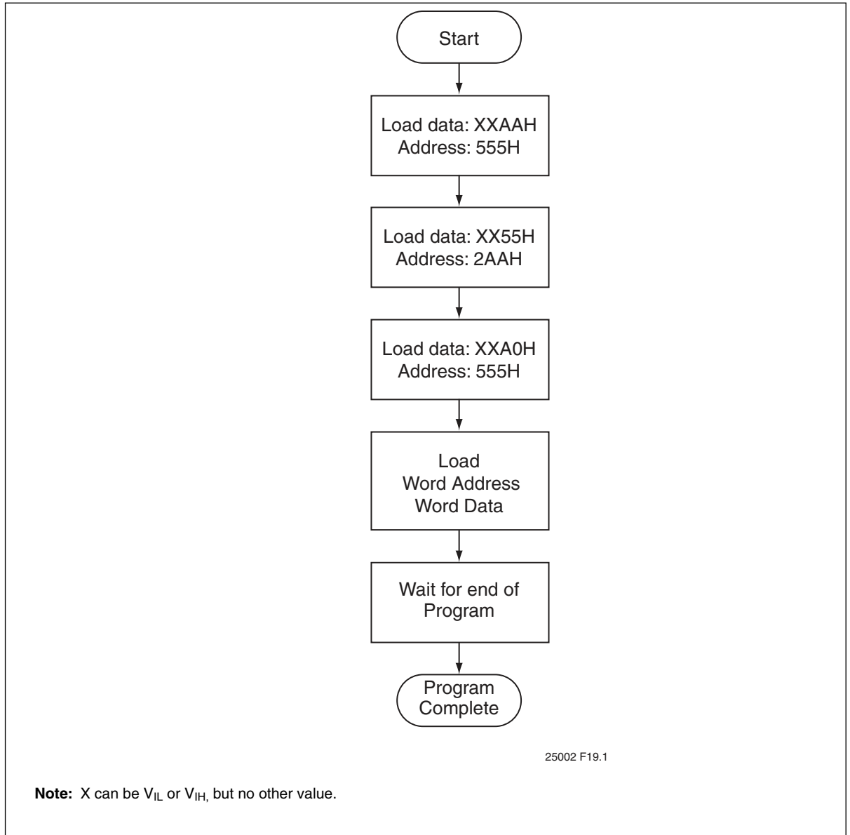
Figure 23: Word-Program Algorithm
