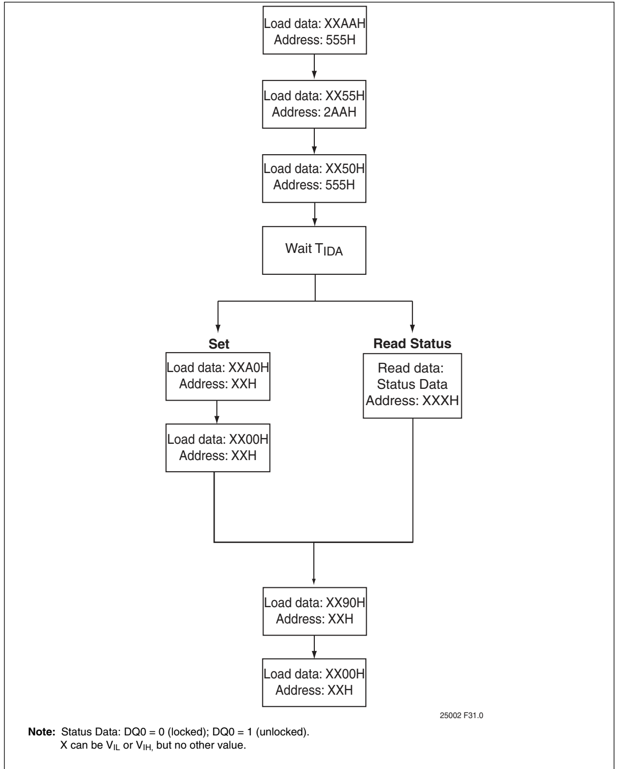
Figure 32: Global Lock of NVPBs
