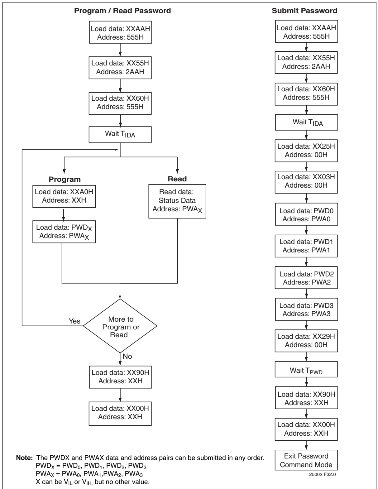
Figure 33: Password Operations (Program, Read, Submit)
