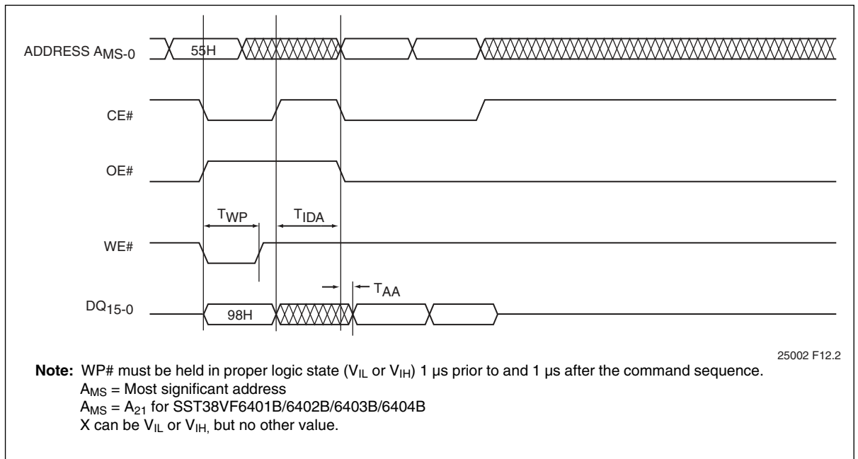
Figure 16: CFI Query Entry and Read
