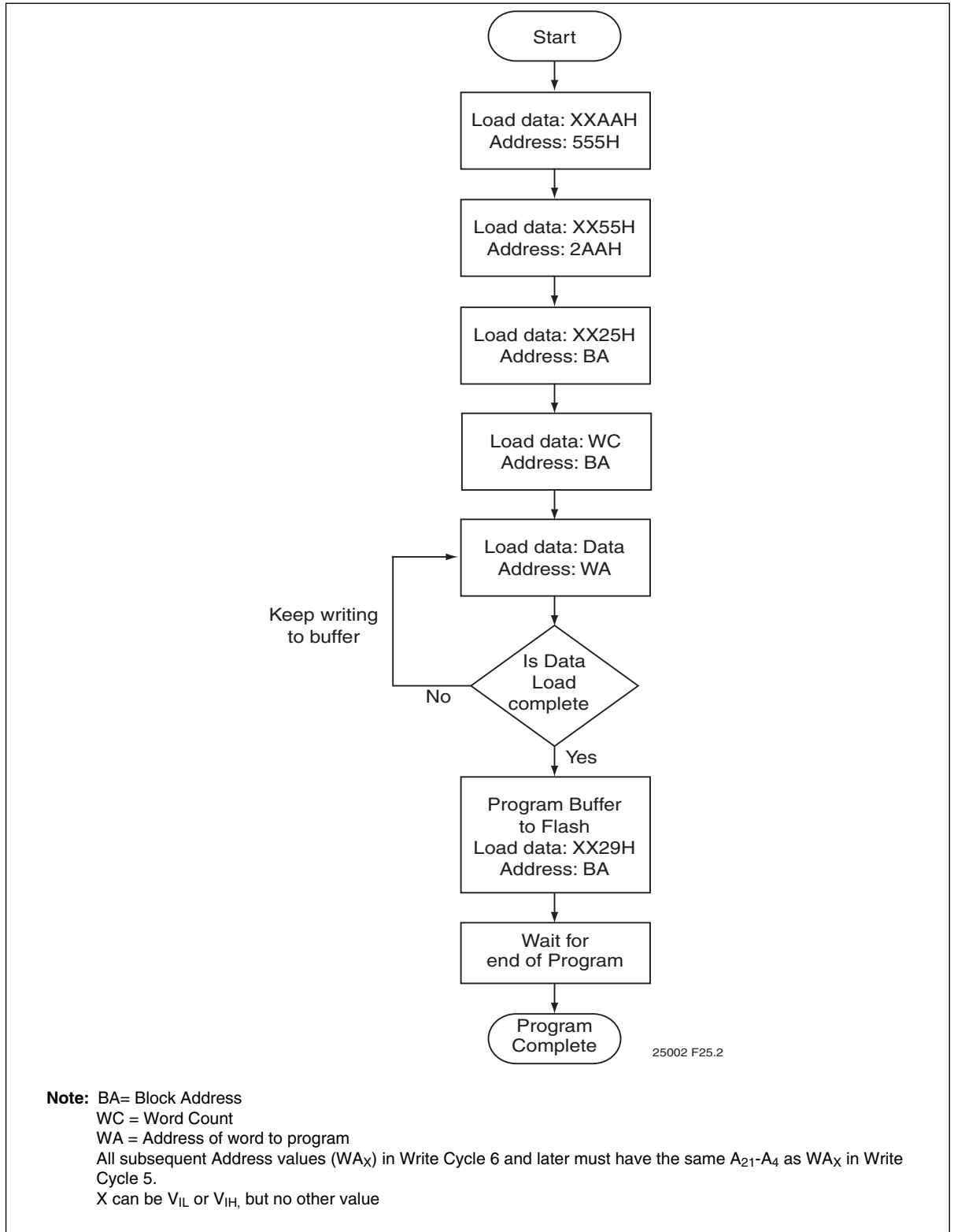
Figure 24: Write-Buffer Programming
