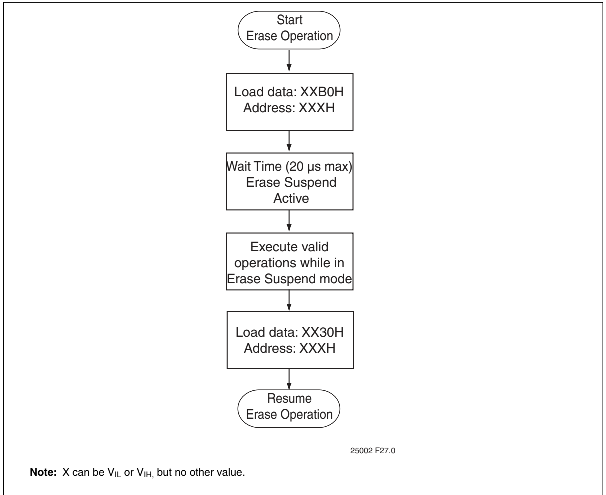
Figure 29: Erase Suspend/Resume
