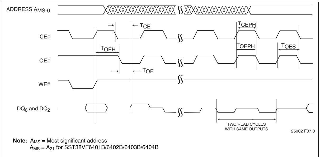
Figure 12: Toggle Bits Timing Diagram
