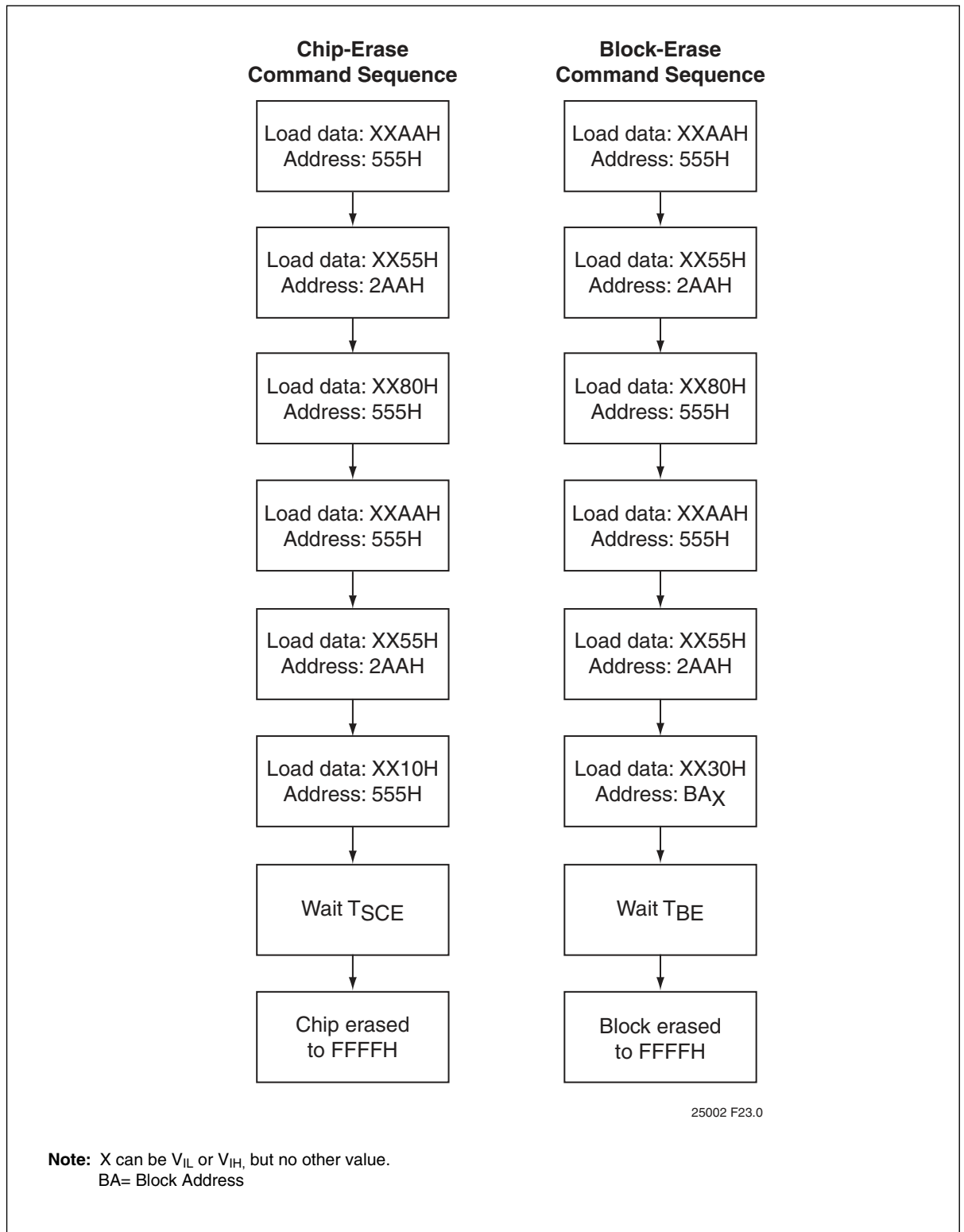
Figure 28: Erase Command Sequence
