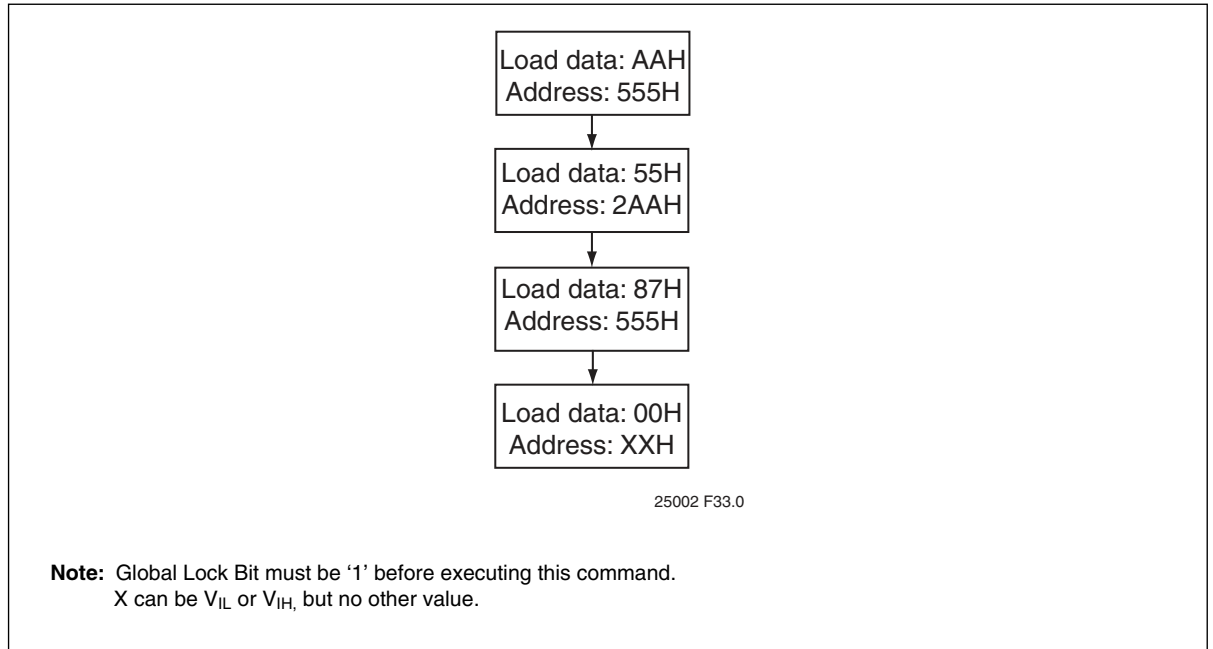
Figure 34: Irreversible Block Lock in Main Array
