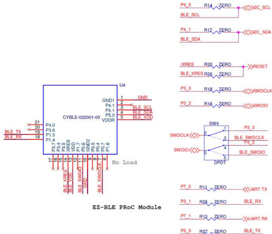
Figure 4-15. EZ-BLE Connections
