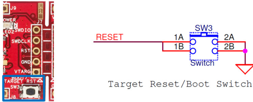
Figure 4-9. Reset/Boot Button
