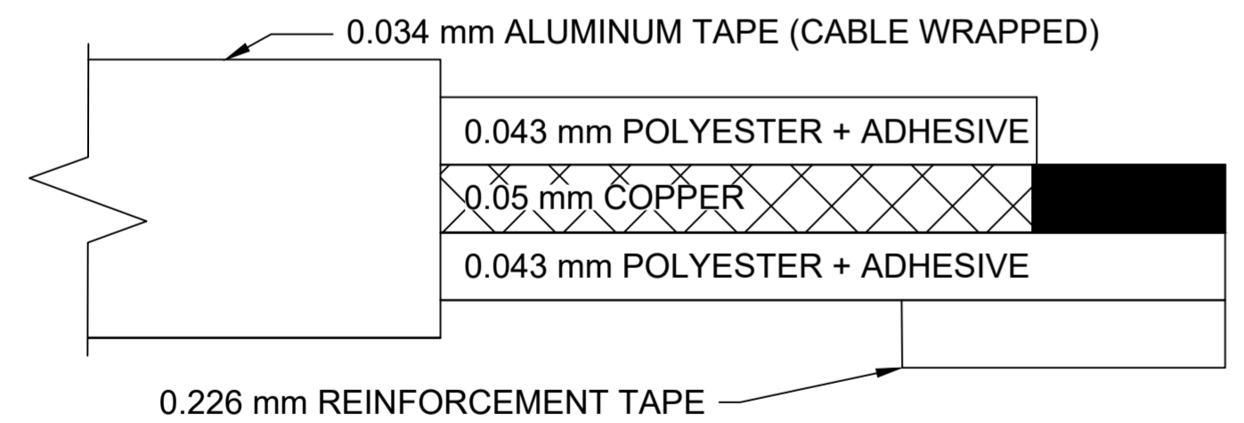
CROSS-SECTION
