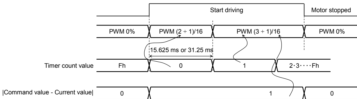
Figure 7.29 PWM Operation 2
