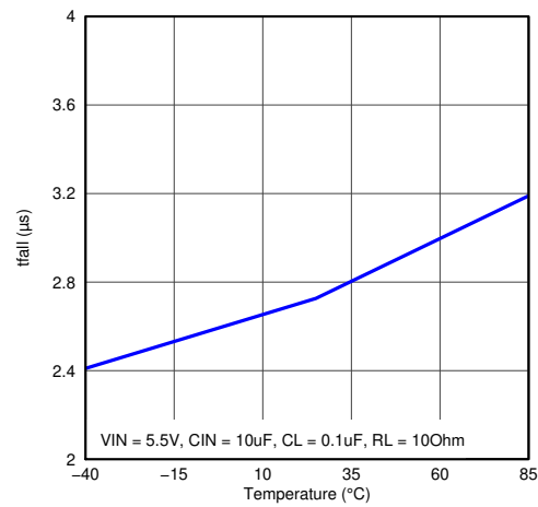
Figure 5-10. t_F vs Temperature ( V_{IN} = 5.5 V )
