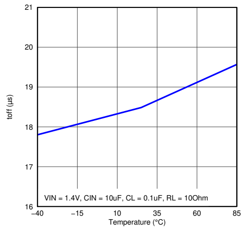
Figure 5-16. t_{OFF} vs Temperature ( V_{IN} = 1.4\text{ V} )
