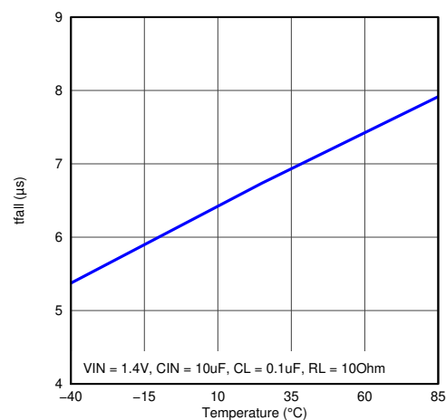
Figure 5-12. t_F vs Temperature ( V_{IN} = 1.4 V )
