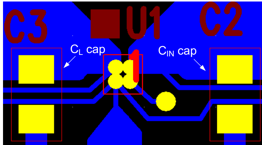
Figure 11-1. Layout Recommendation
