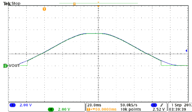
Figure 9-2. UVLO Response
