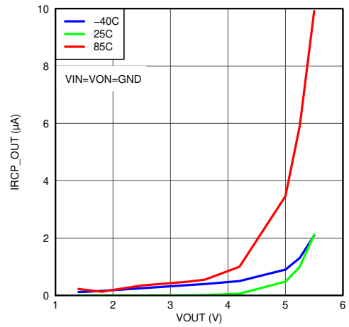
Figure 5-8. I_{RCP(Leak)} vs V_{OUT} (Measured on V_{OUT} )
