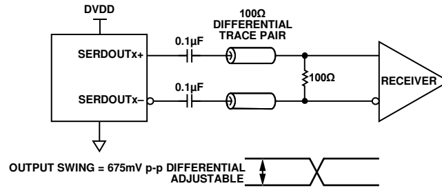
Figure 88. AC-Coupled Digital Output Termination Example
