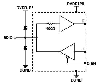
Figure 50. SDIO Input/Output
