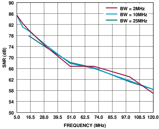
Figure 34. SNR vs. Sliding IF
