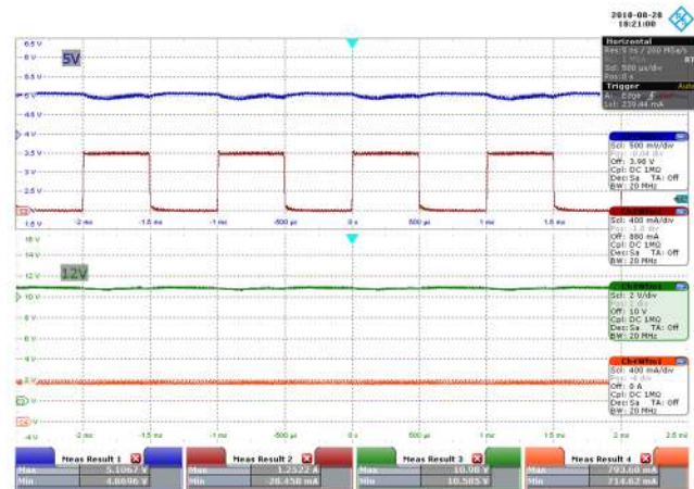
Figure 28 – 115 VAC 60 Hz.
