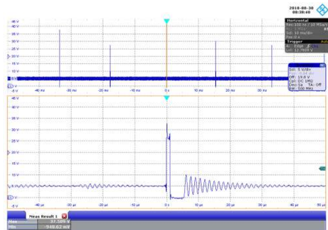
Figure 74 – 277 VAC 50 Hz, No-Load. CH1: 5 V FWL_DIODE , 5 V / div., 10 ms / div. Zoom: 10 \mu s / div. 5 V PIV MAX = 37.589 V.
