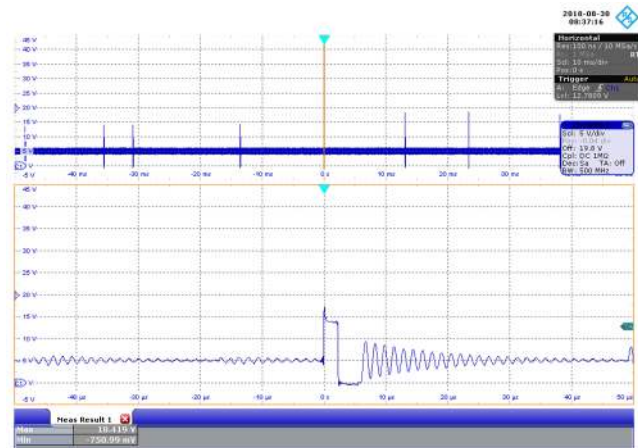
Figure 72 – 115 VAC 60 Hz, No-Load. CH1: 5 V FWL_DIODE , 5 V / div., 10 ms / div. Zoom: 10 \mu s / div.. 5 V PIV MAX = 18.419 V
