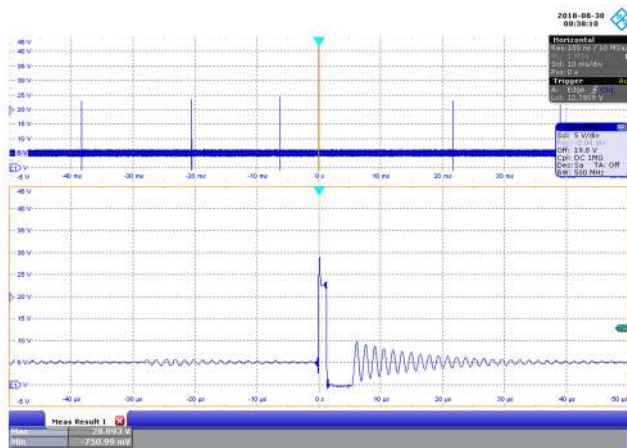
Figure 73 – 230 VAC 50 Hz, No-Load. CH1: 5 V FWL_DIODE , 5 V / div., 10 ms / div. Zoom: 10 \mu s / div. 5 V PIV MAX = 28.893 V.
