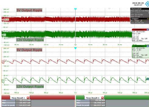
Figure 118 – 85 VAC 60 Hz, 50% Load. CH2: 5 V_{OUT} , 40 mV / div., 10 ms / div. CH3: 12 V_{OUT} , 40 mV / div., 10 ms / div. Zoom: 40 \mu s / div. 5 V Output Ripple = 64.822 mV. 12 V Output Ripple = 86.957 mV.
