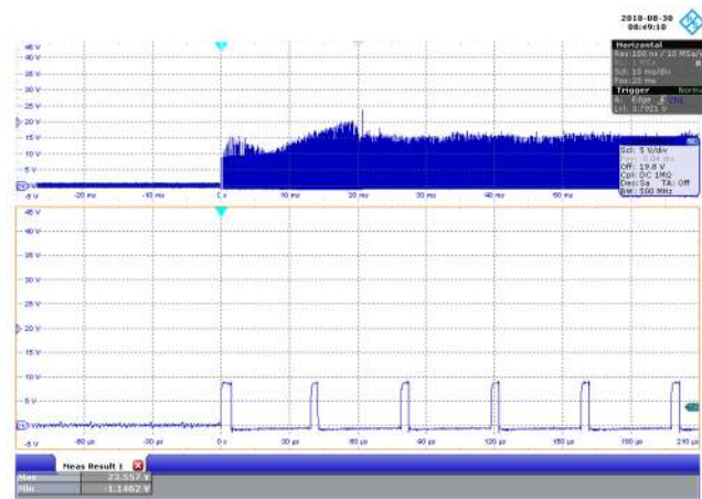
Figure 76 – 115 VAC 60 Hz, Full Load. CH1: 5 V F WL _DIODE , 5 V / div., 10 ms / div. Zoom: 30 µs / div. 5 V PIV MAX = 23.557 V.
