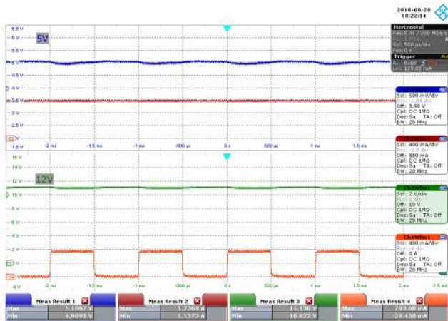
Figure 31 – 85 VAC 60 Hz.
