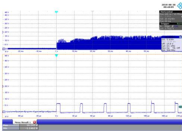
Figure 75 – 85 VAC 60 Hz, Full Load. CH1: 5 V F WL _DIODE , 5 V / div., 10 ms / div. Zoom: 30 µs / div. 5 V PIV MAX = 16.245 V.
