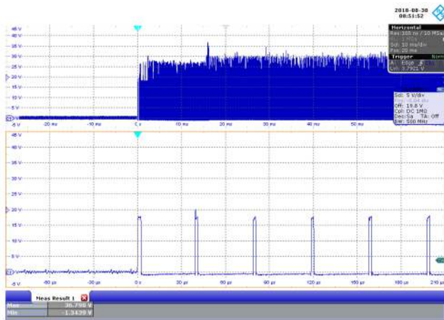
Figure 77 – 230 VAC 50 Hz, Full Load. CH1: 5 V F WL _DIODE , 5 V / div., 10 ms / div. Zoom: 30 µs / div. 5 V PIV MAX = 36.798 V.
