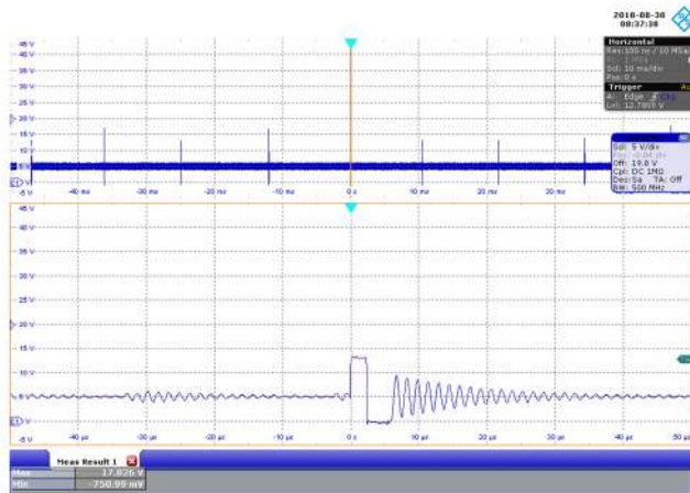
Figure 71 – 85 VAC 60 Hz, No-Load. CH1: 5 V FWL_DIODE , 5 V / div., 10 ms / div. Zoom: 10 \mu s / div. 5 V PIV MAX = 17.826 V.
