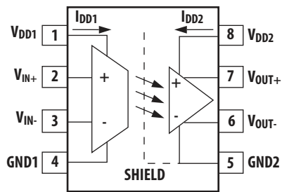
Figure 1: Functional Diagram
