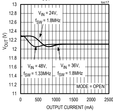
LOAD REGULATION V_{OUT} = 12V , PFM MODE
