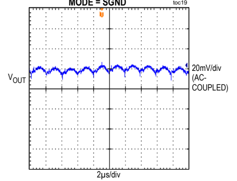
OUTPUT VOLTAGE RIPPLE V_{IN} = 24V , V_{OUT} = 3.3V , I_{OUT} = 2.5A , MODE = SGND
