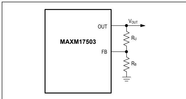
Figure 1. Adjustable Output Voltage
