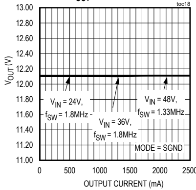
LOAD REGULATION V_{OUT} = 12V , PWM MODE
