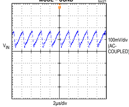
INPUT VOLTAGE RIPPLE
