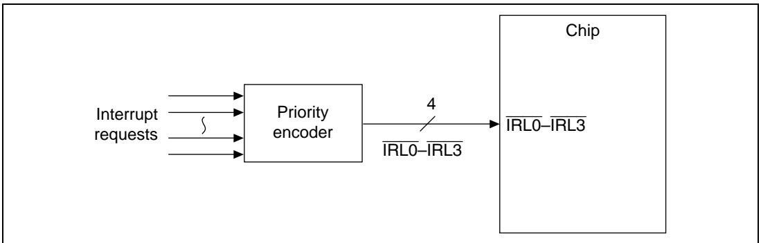
Figure 5.3 Example of Connections for Auto-Vector Mode Interrupts
