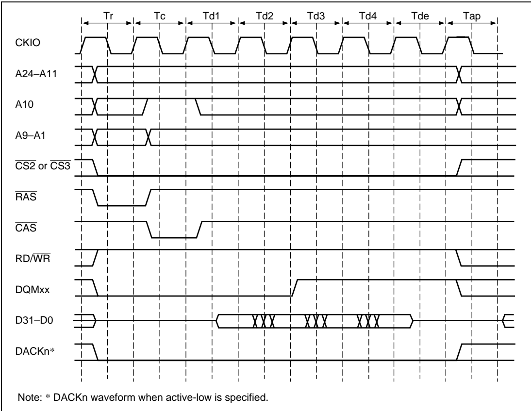
Figure 7.21 (a) Single Read Timing (Auto-Precharge) Except t_{Eyc} : t_{Pyc} 1:1
