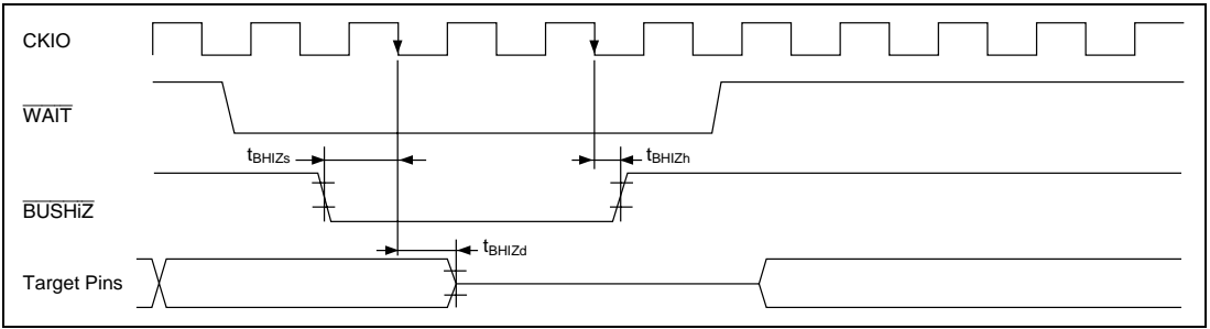
Figure 21.80 \overline{\text{BUSHiZ}} Bus Timing
