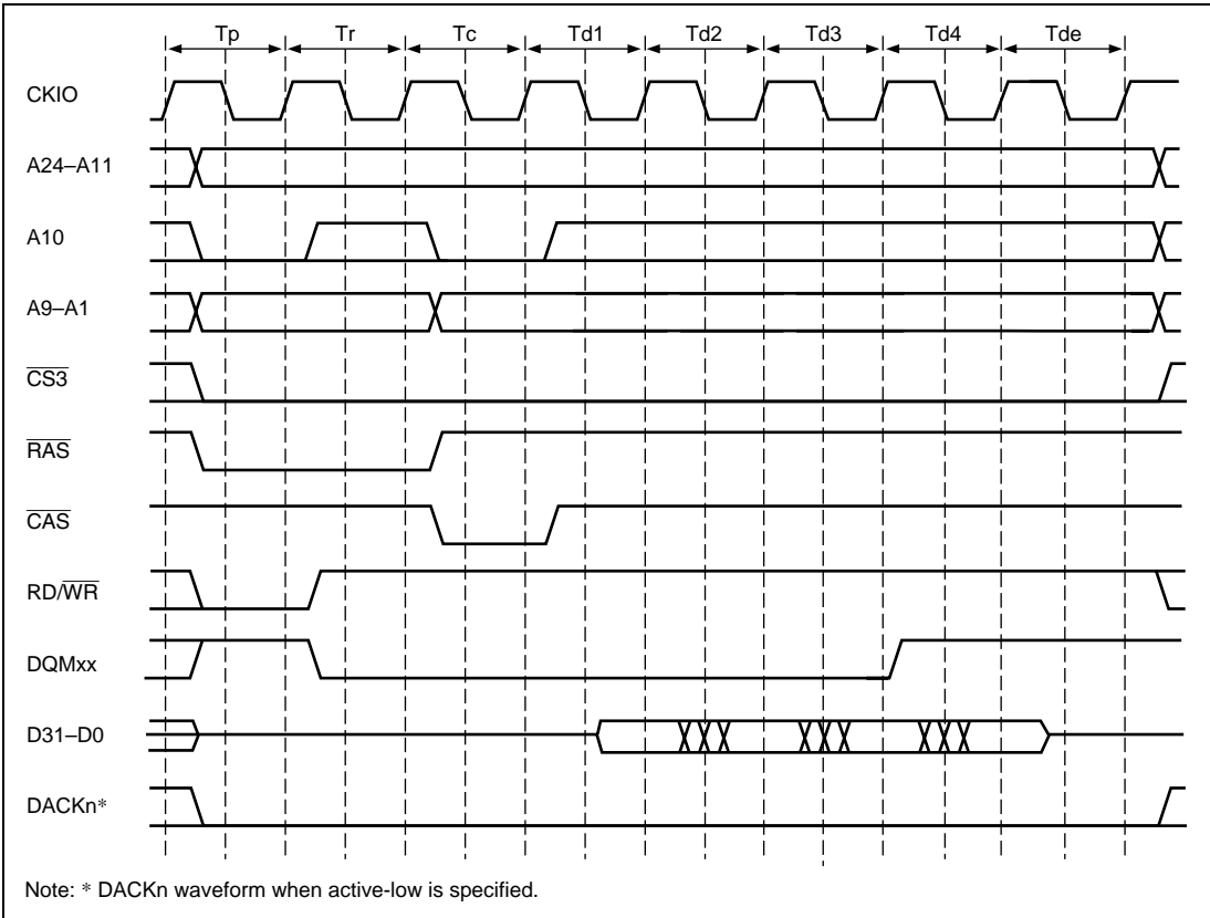
Figure 7.26 (a) Burst Read Timing (Bank Active, Different Row Addresses) Except t_{E_{eye}}:t_{P_{cyc}} 1:1
