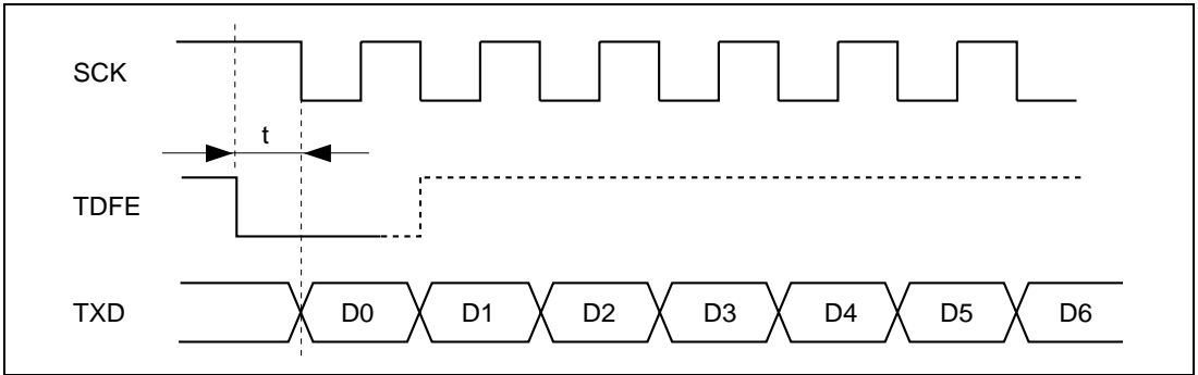
Figure 14.26 Example of Synchronous Transmission by DMAC
