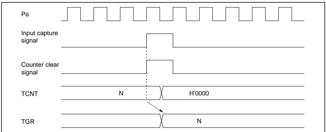
Figure 16.35 Counter Clear Timing (Input Capture)
