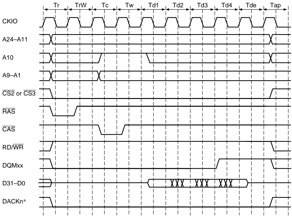
Figure 7.20 (a) Burst Read Wait Specification Timing (Auto-Precharge) Except t_{Eye} : t_{Peye} 1:1
