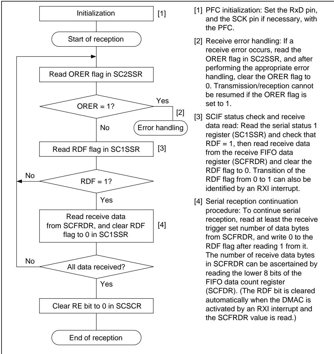
Figure 14.20 Sample Serial Reception Flowchart (1)
