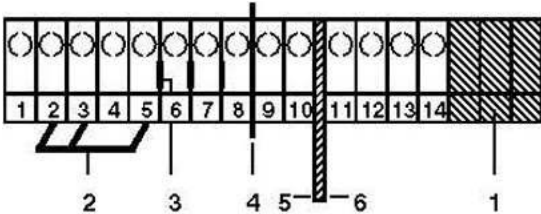
Circuit diagram
