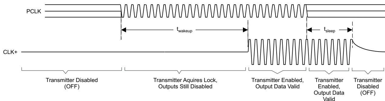
Figure 14. Standby Detection
