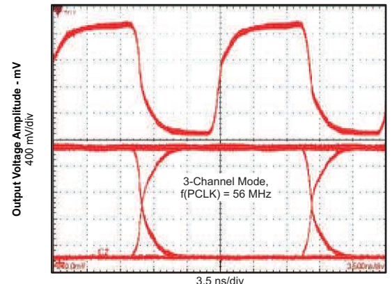
Response With 10-pF Load Figure 30.
