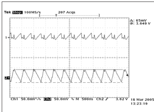
Figure 5. Ripple 1X Flash 400mA CH1=Vin, CH2=Vout, V_{in}=4.2\text{V} , C_{in}=4.7\mu\text{F} , C_{FC}=0.47\mu\text{F} , C_{out}=2.2\mu\text{F}
