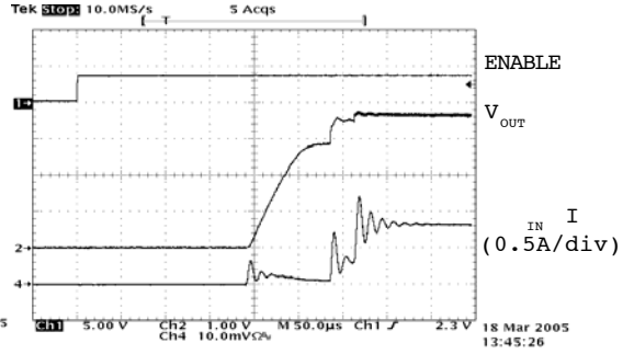
Figure 16. Startup Flash, V_{in}=3.6V , V_{out}=3.5V C_{in}=4.7\mu F , C_{FC}=0.47\mu F , C_{out}=2\mu F
