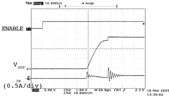
Figure 15. Startup Torch, V_{in}=3.6V , V_{out}=3.1V C_{in}=4.7\mu F , C_{FC}=0.47\mu F , C_{out}=2\mu F
