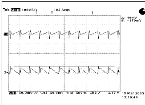
Figure 7. Ripple 1X Torch 150mA CH1=Vin, CH2=Vout, V_{in}=4.2\text{V} , C_{in}=4.7\mu\text{F} , C_{FC}=0.47\mu\text{F} , C_{out}=2.2\mu\text{F}
