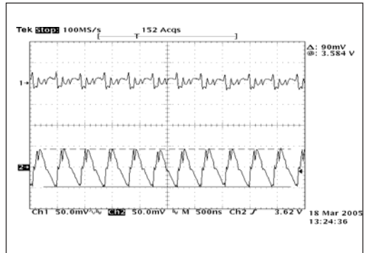
Figure 6. Ripple 2X Flash 400mA CH1=Vin, CH2=Vout, V_{in}=3.6\text{V} , C_{in}=4.7\mu\text{F} , C_{FC}=0.47\mu\text{F} , C_{out}=2.2\mu\text{F}
