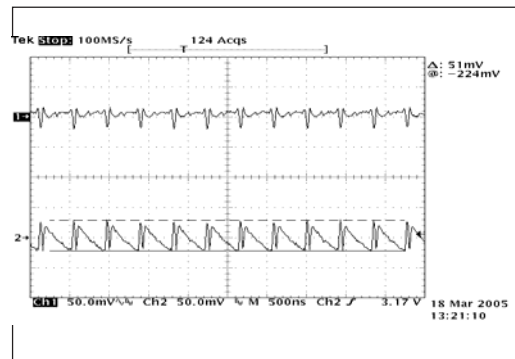
Figure 8. Ripple 2X Torch 150mA CH1=Vin, CH2=Vout, V_{in}=3.0\text{V} , C_{in}=4.7\mu\text{F} , C_{FC}=0.47\mu\text{F} , C_{out}=2.2\mu\text{F}
