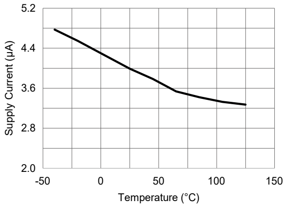
Figure 11. Supply current versus temperature ( V_{CC} = 3\text{ V} )
