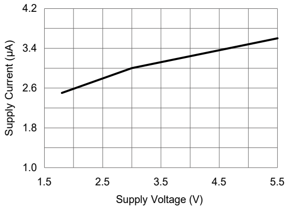
Figure 7. Supply current versus supply voltage ( T_A=25^\circ\text{C} )
