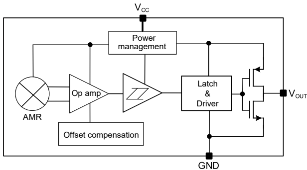
Figure 1. Block diagram
