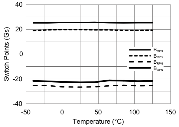
Figure 10. Switch points versus temperature ( V_{CC} = 3\text{ V} )
