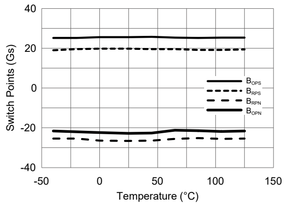
Figure 12. Switch points versus temperature ( V_{CC} = 3\text{ V} )
