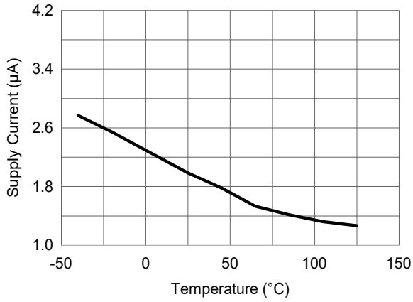
Figure 9. Supply current versus temperature ( V_{CC} = 3\text{ V} )
