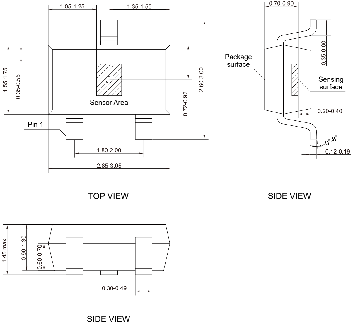
Figure 15. Package outline of SOT23-3 (unit: mm)
