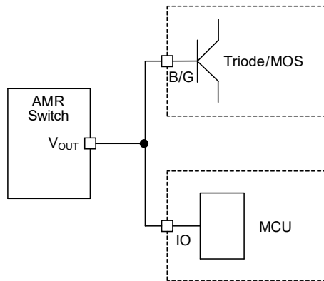
Figure 14. Application diagram for driving power load
