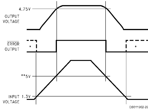
Error Output Timing Diagram
