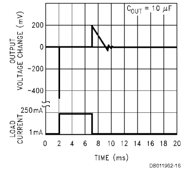
Load Transient
