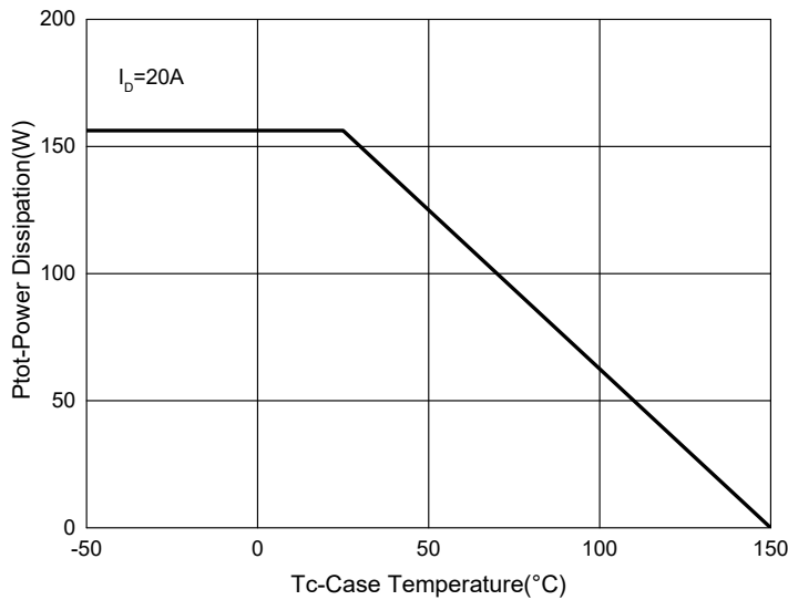
Fig. 9 - Power Dissipation
