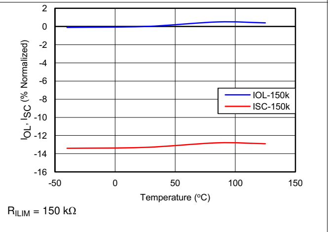
Figure 16. I_{OL} , I_{SC} vs Temperature
