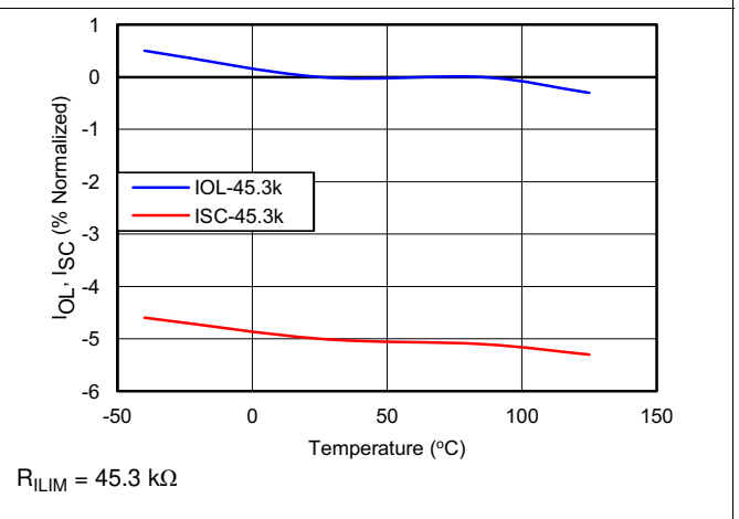
Figure 18. I_{OL} , I_{SC} vs Temperature
