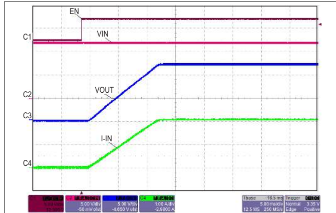
C dVdT = 1nF, C OUT = 10 μF, R OUT = 5.7Ω
