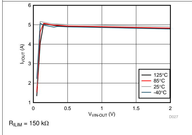
Figure 15. I_{VOUT} vs V_{VIN-OUT}
