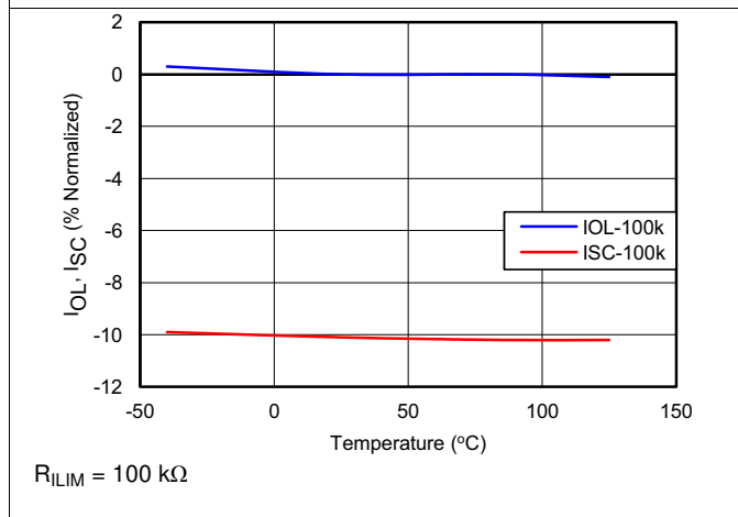
Figure 17. I_{OL} , I_{SC} vs Temperature
