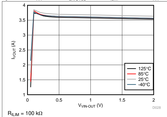
Figure 13. I_{VOUT} vs V_{VIN-OUT}
