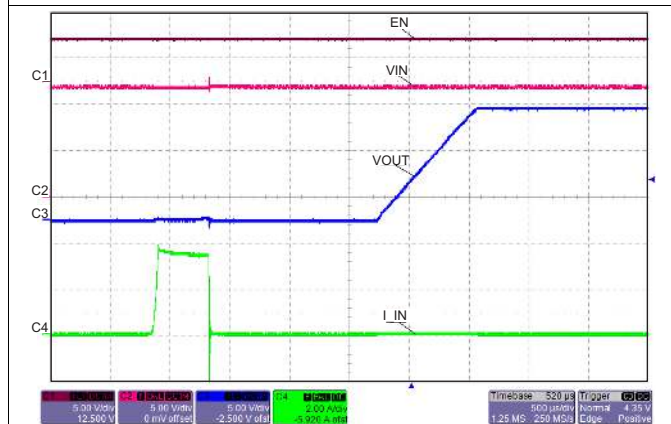
TPS259241
