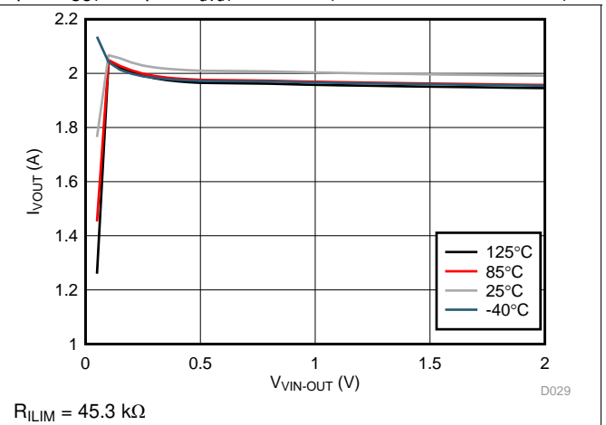
Figure 14. I_{VOUT} vs V_{VIN-OUT}
