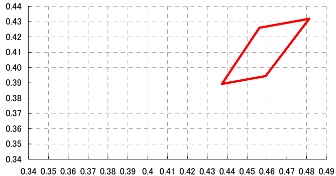
Chromaticity coordinate
