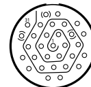
18-31 31 Size 20 Contacts
