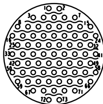
17-23 73 Size 23 Contacts
