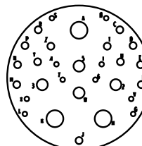
25-21 3 Size 8 Twinax Contacts 4 Size 12 Coax Contacts 13 Size 16 Contacts 10 Size 20 Contacts
