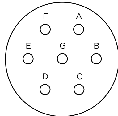
16-1 7 Size 16 Contacts
