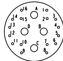
17-20 4 Size 12 Contacts 16 Size 22D Contacts
