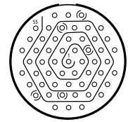
22-55 55 Size 20 Contacts
