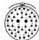
20-39 37 Size 20 Contacts 2 Size 16 Contacts
