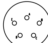
15-05 5 Size 16 Contacts
