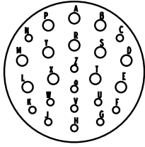
25-24 12 Size 12 Contacts 12 Size 16 Contacts
