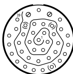
20-39 37 Size 20 Contacts 2 Size 16 Contacts
