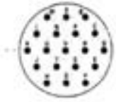
14-19 19 Size 20 Contacts
