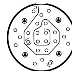
20-28 24 Size 20 Contacts 4 Size 12 Contacts
