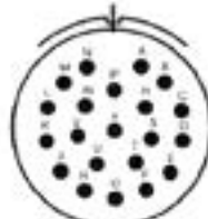
22-21 21 Size 16 Contacts
