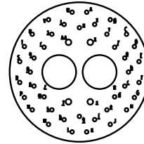
25-91 2 Size 8 Twinax Contacts 4 Size 16 Contacts 40 Size 20 Contacts
