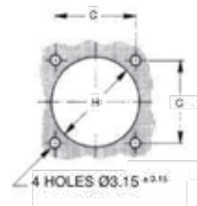
Panel Boring
