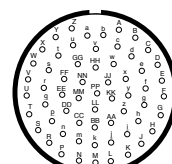
24-61 61 Size 20 Contacts
