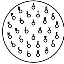
25-29 29 Size 16 Contacts
