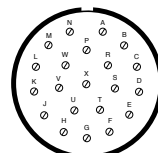
22-21 21 Size 16 Contacts
