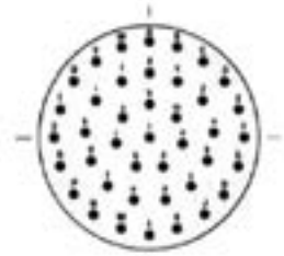
20-41 41 Size 20 Contacts
