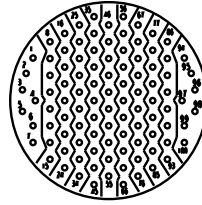
23-35 100 Size 22D Contacts
