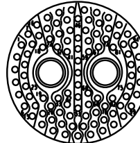
25-07* 2 Size 8 Twinax Contacts 97 Size 22D Contacts
