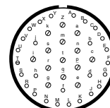
22-41 27 Size 20 Contacts 14 Size 16 Contacts
