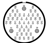
61-949 46 Size 20 Contacts 3 Size 8 Contacts
