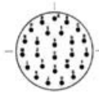
16-26 26 Size 20 Contacts
