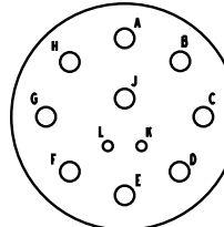
25-11 9 Size 10 Contacts 2 Size 20 Contacts
