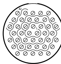
28-42 42 Size 16 Contacts *
