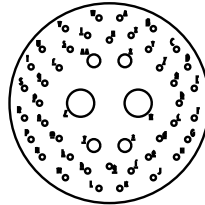
25-90* 2 Size 8 Twinax Contacts 4 Size 16 Contacts 40 Size 20 Contacts
