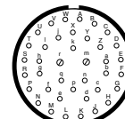
20-39 37 Size 20 Contacts 2 Size 16 Contacts
