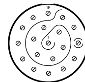
22-19 19 Size 16 Contacts
