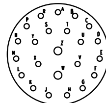
17-99 2 Size 16 Contacts 21 Size 20 Contacts
