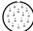
20-16 16 Size 16 Contacts
