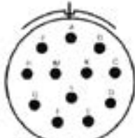
22-12 12 Size 12 Contacts
