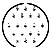
24-19 19 Size 12 Contacts
