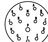
15-15 14 Size 20 Contacts
