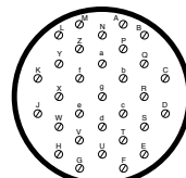
24-31 31 Size 16 Contacts
