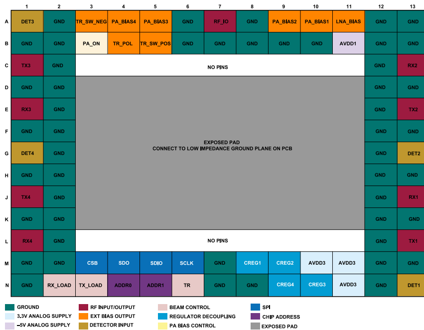
Figure 9. Pin Configuration, Color Coded (Top View)
