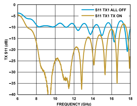
Figure 105. Transmit Return Loss While Powered Up and Powered Down
