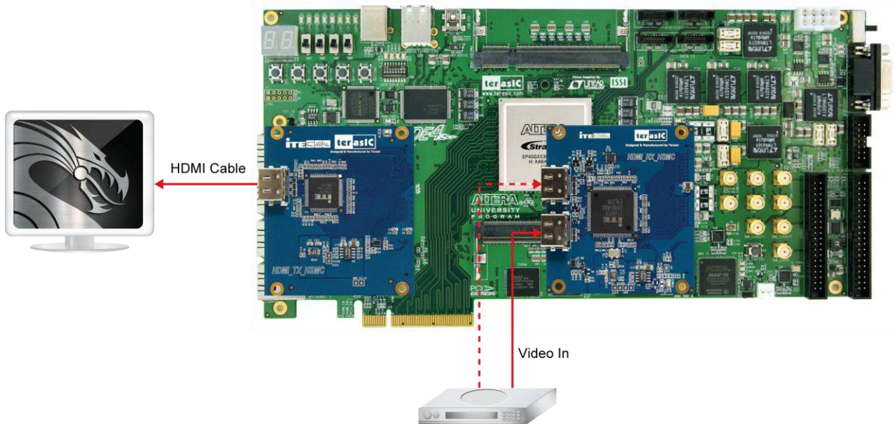
Figure 3-1 Loopback HDMI_RX to HDMI_TX Demonstration Setup
