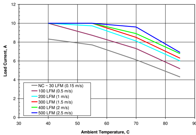
Figure 1. Available load current vs. ambient air temperature and airflow rates for SQE48T10120 converter mounted vertically with air flowing from pin 3 to pin 1, MOSFET temperature \leq 120 °C, V_{in} = 48 V.
