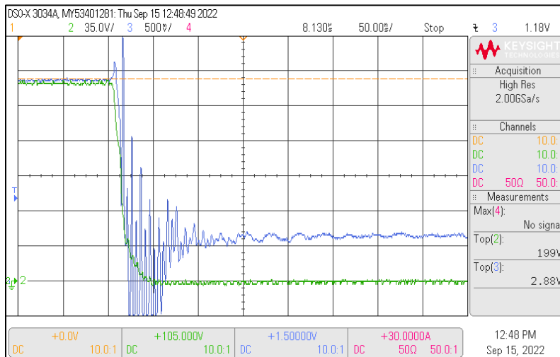
Figure: Double-pulse test: 200VDC, 45A. Green trace: Drain-Source Voltage. Blue trace: Tell-i VON1k5Vm output. Magenta trace: Inductor current. Tell-i VON1k5Vm settlement time: <50nsec. The device under test: GaN GS6651B.
