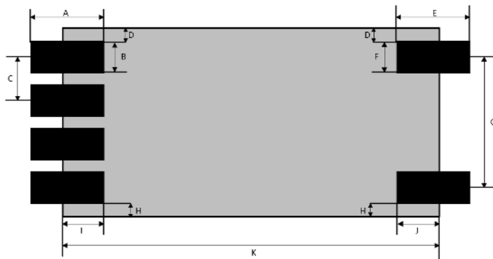
Figure. Bottom footprint with pad measurements for hand-soldering
