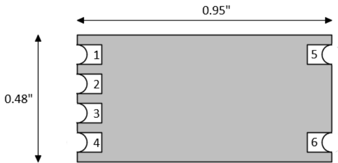
Figure. Bottom footprint: 0.95" x 0.48"
