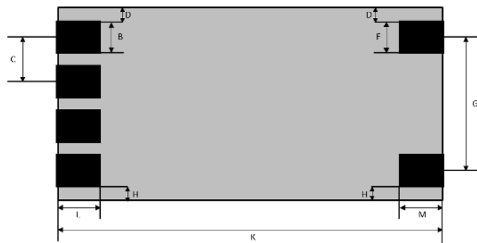
Figure. Bottom footprint with pad measurements for reflow-soldering
