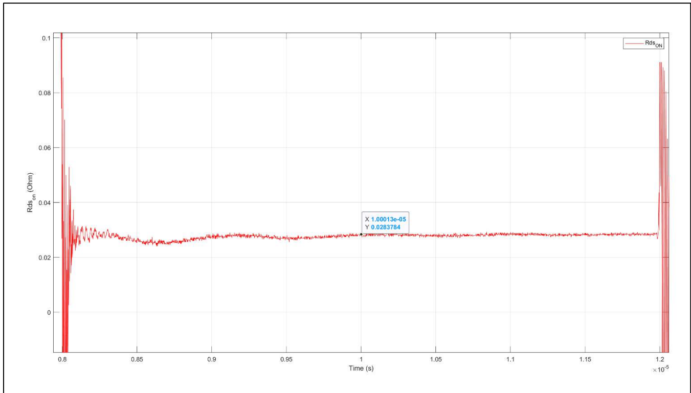
Figure: Red trace: 2 nd Pulse R_{DSON} measurement of DUT. The device under test: GaN Systems 650V GaN GS6651B approximate R_{DSON} \approx 25m\Omega . Tell-i VON1k5Vm R_{DSON} \approx 28m\Omega .
