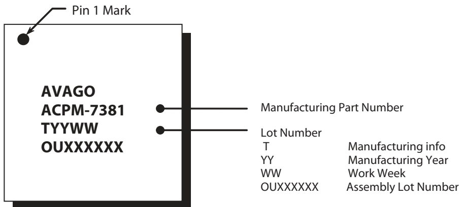
Figure 14. Marking Specifications
