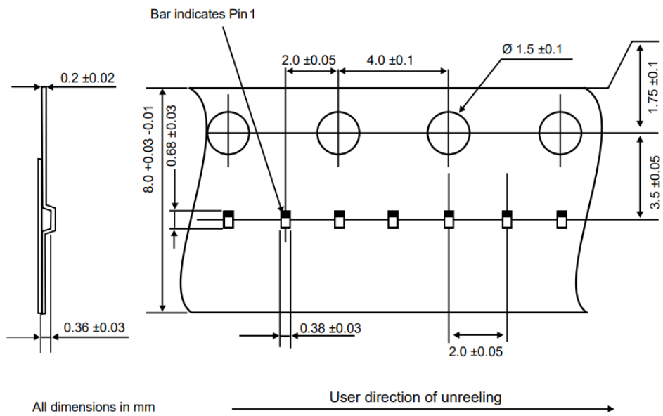
Figure 9. Tape and reel specification (in mm)
