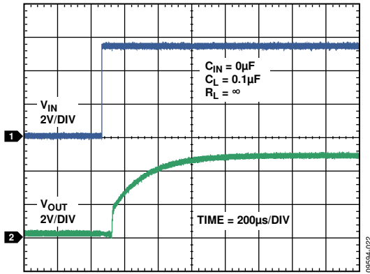
Figure 22. ADR3550 Start-Up Response
