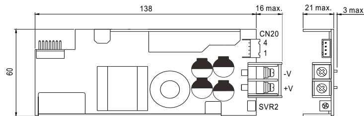
Output Connector(CN20) : JST B4B-XH or equivalent
