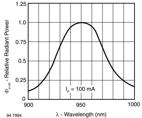
Fig. 9 - Relative Radiant Power vs. Wavelength
