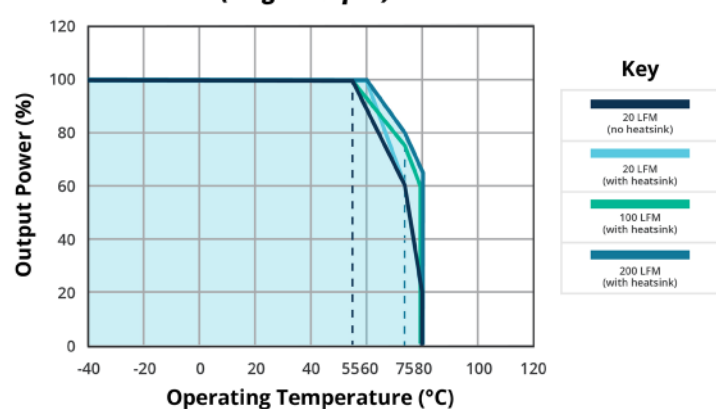
TEMPERATURE DERATING CURVE (single output)
