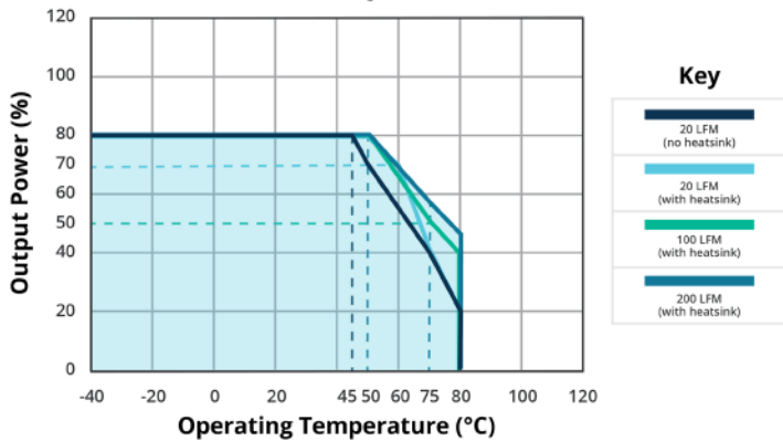
TEMPERATURE DERATING CURVE (dual output)
