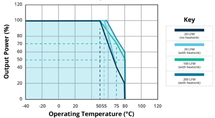
TEMPERATURE DERATING CURVE (dual output)
