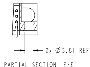
PARTIAL SECTION E-E
