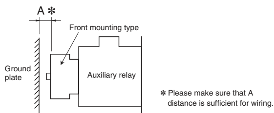
Diagram 3. Mounting space
