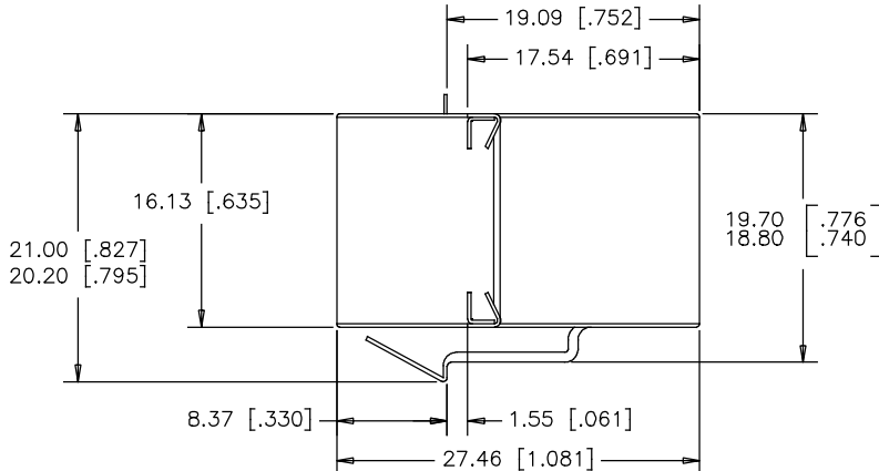
SIDE VIEW
