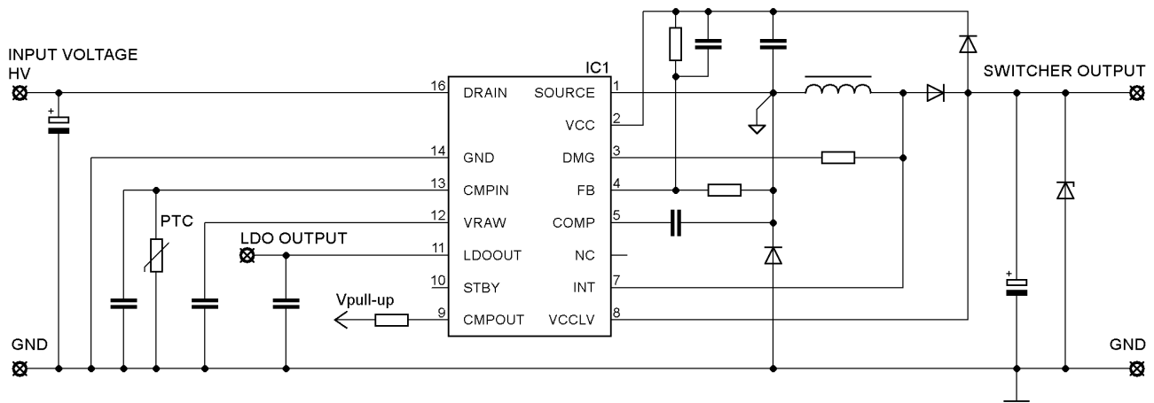
Figure 1. Application Schematic
